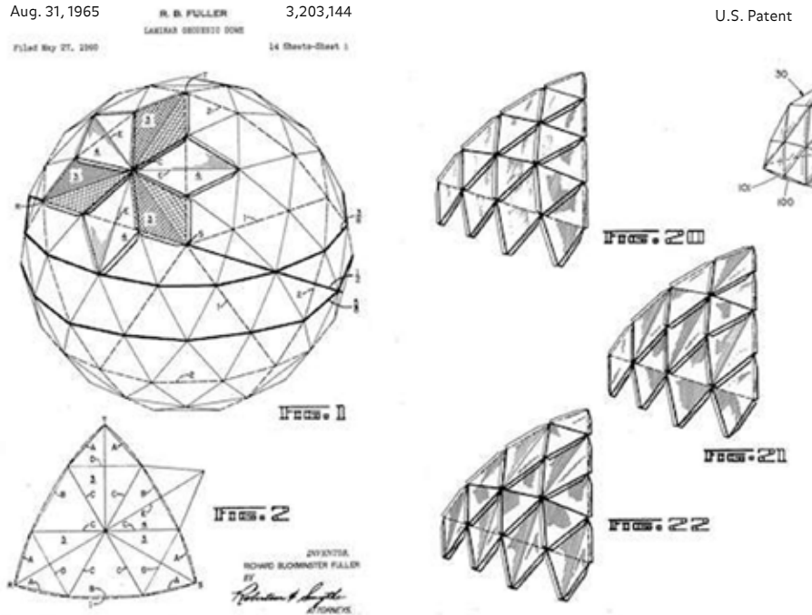
Figure 21: Buckminster Fuller, Geodesic dome (Construction concept development dwgs) – 1965
